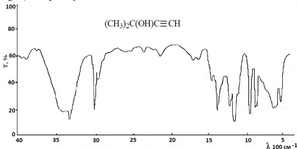
Fig.1. IR-spectrum dimethylethynylcarbinol.
