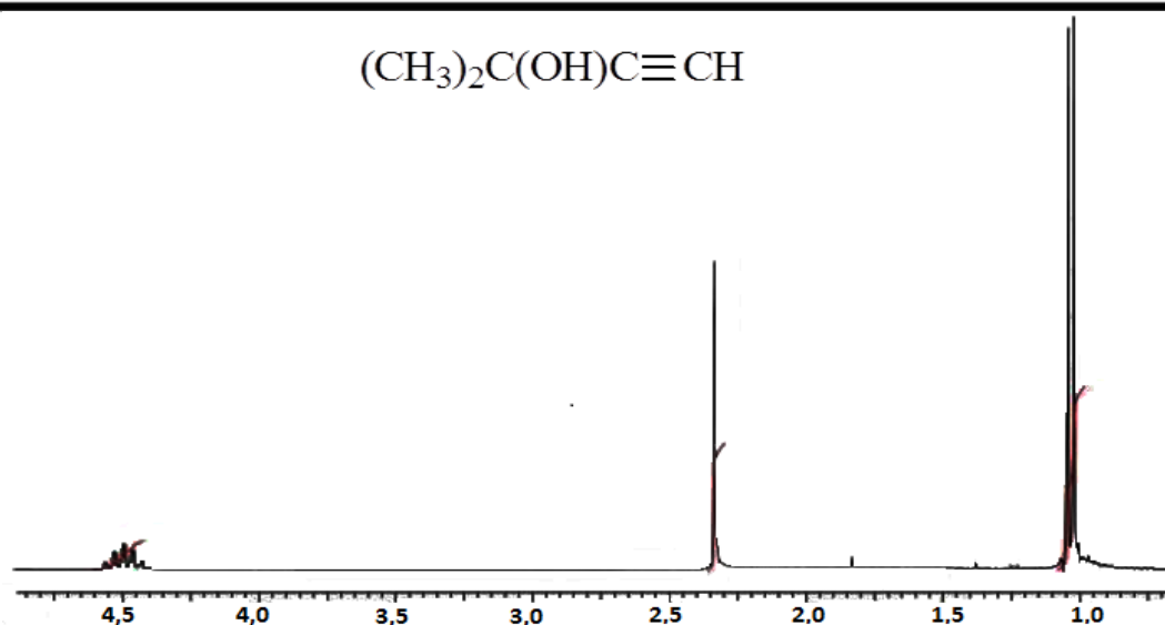
Fig.2. PMR 1H – spectrum dimethylethynylcarbinol
