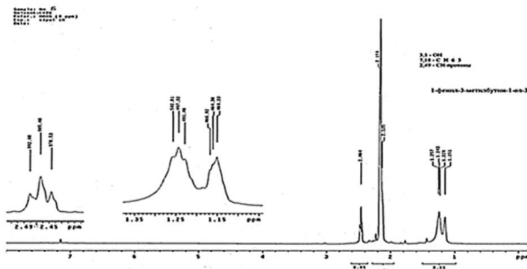
Fig.3. PMR 1H- spectrum 1-phenyl-3-methylbutin-1-ola-3
